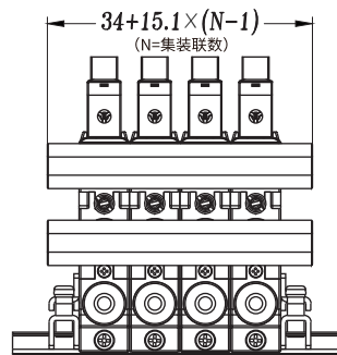
(multi-side view)
