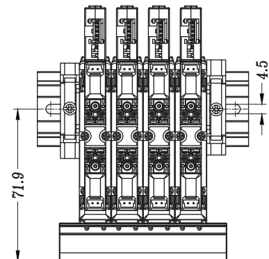
(Multi-top view)
