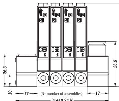
(multi-side view)
