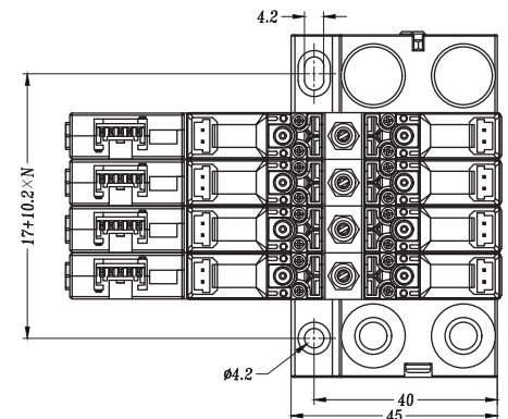
(Multi-top view)
