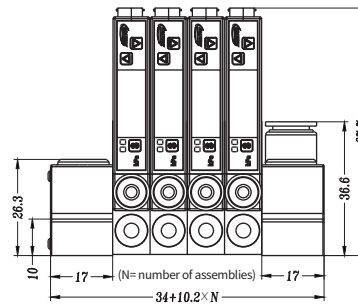
(multi-side view)
