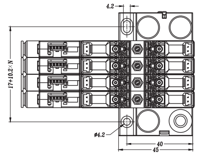
(Multi-top view)
