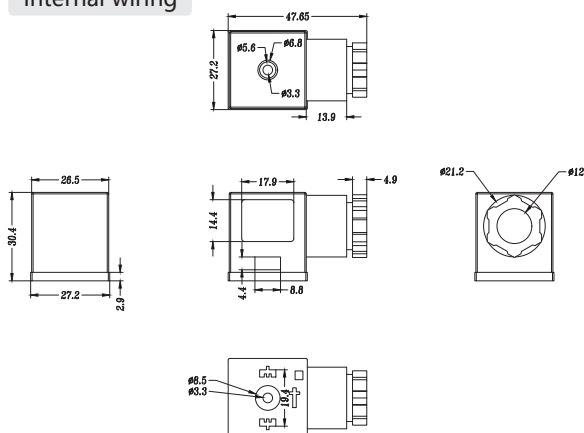
Internal wiring
